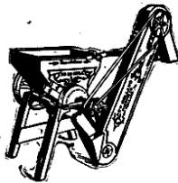
MODEL NO. 10 AND NUMBER 12 FEED MILL WITH ELEVATOR AND TWO-SPOUT RABBIT ATTACHMENT
